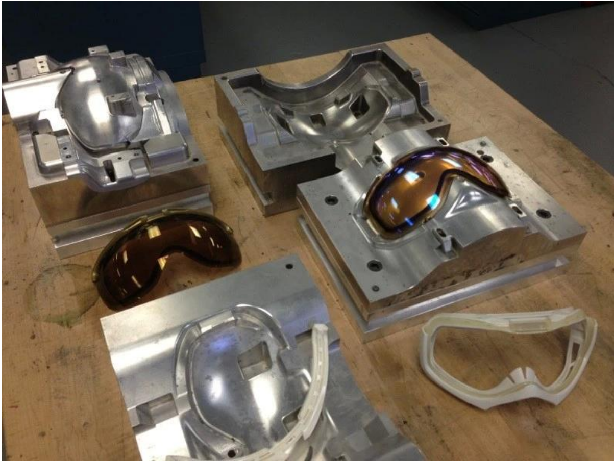
Open EPS mold
